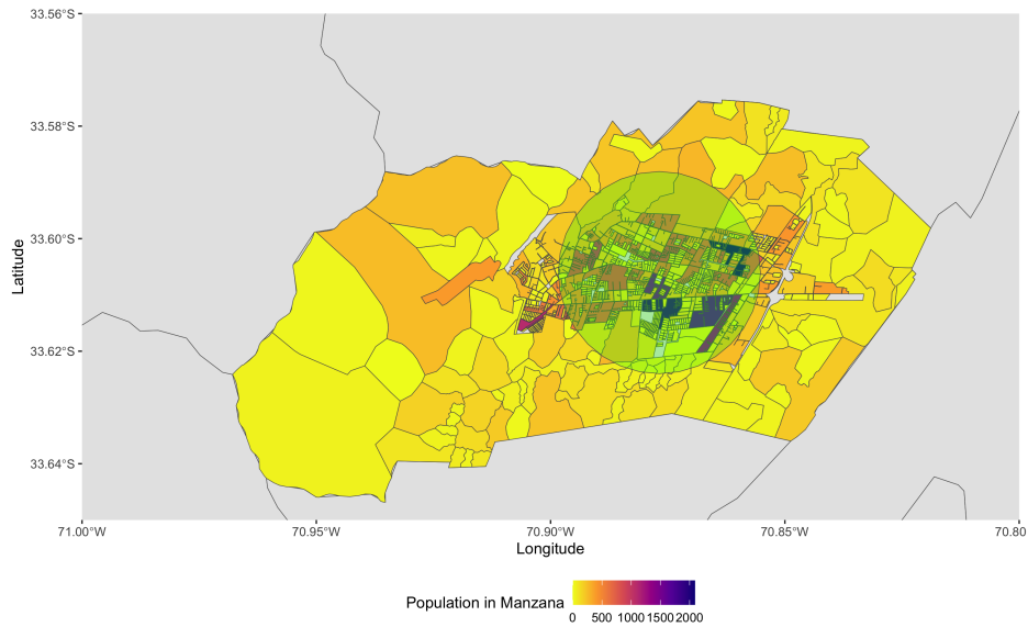
Figure C.4: Population weighted centroids, high accuracy – Peñaflores
