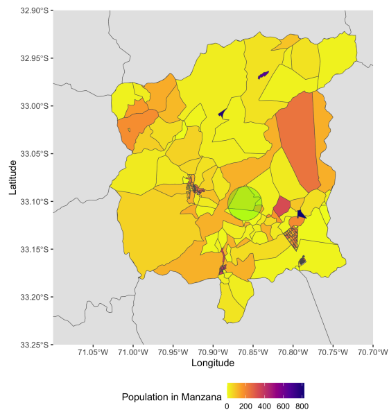
Figure C.5: Population weighted centroids, low accuracy – Tiltil
