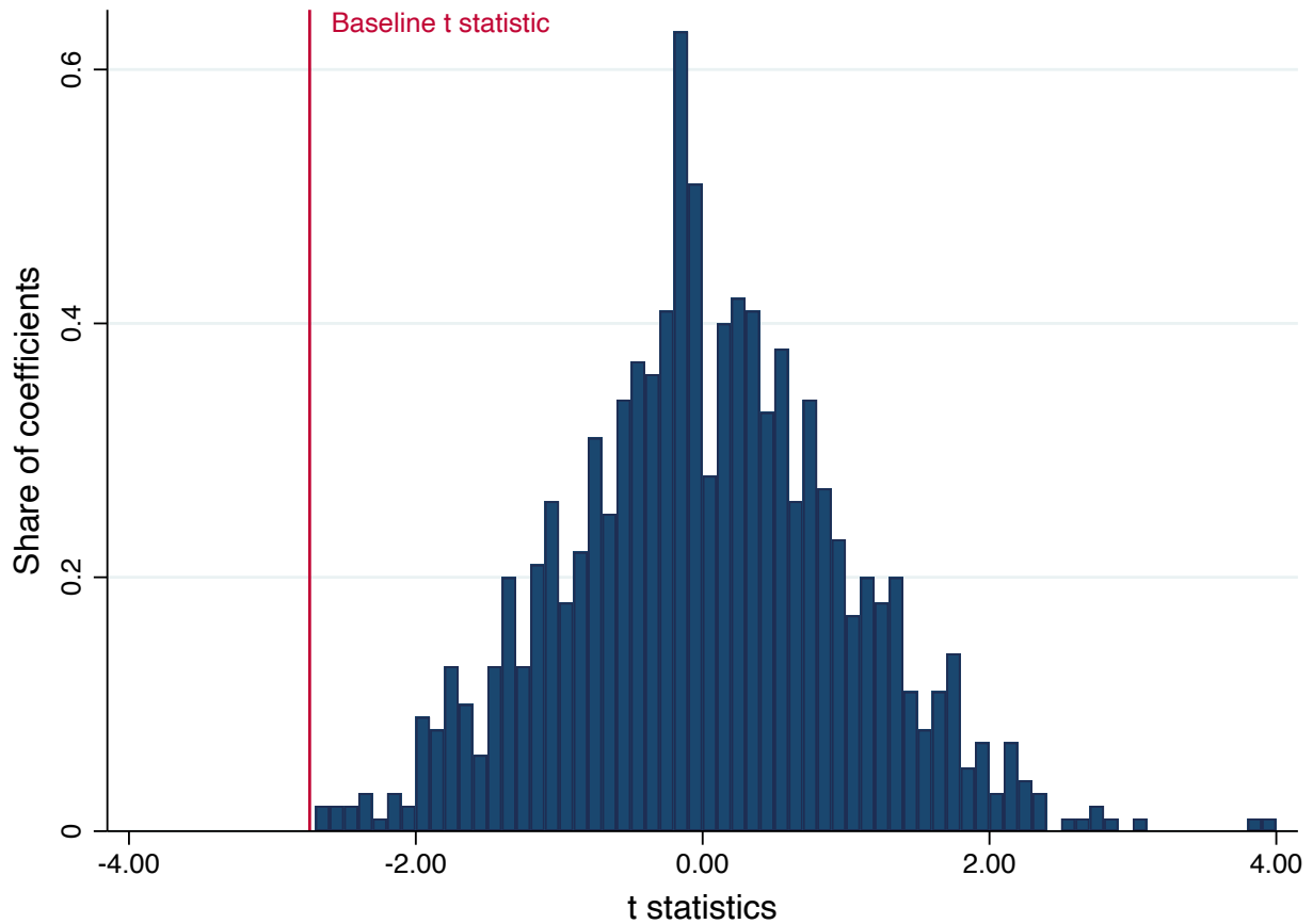
Figure C.3: Placebo with randomization within year
