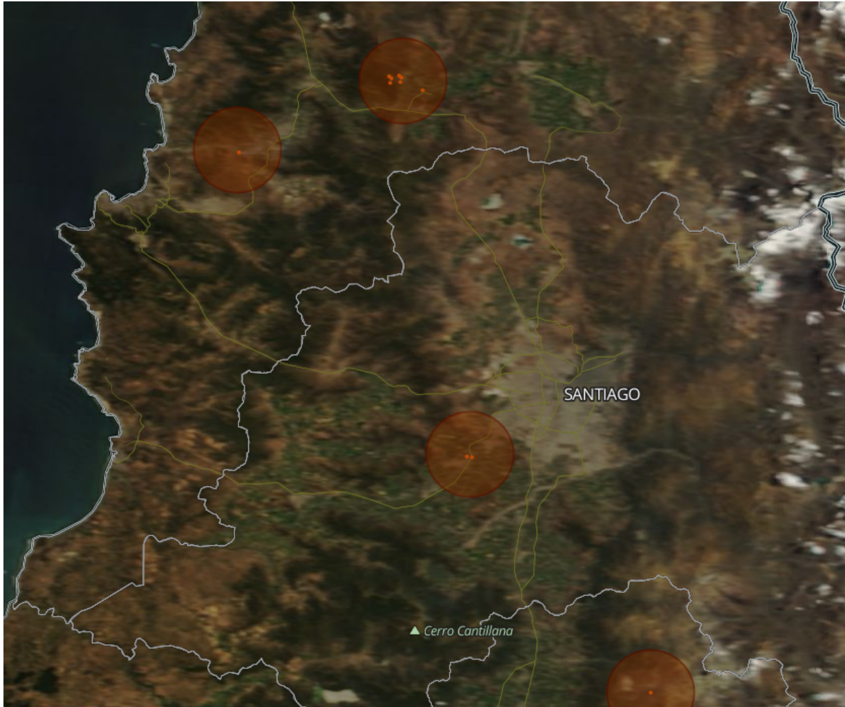
Figure C.1: Measuring exposure to fire
